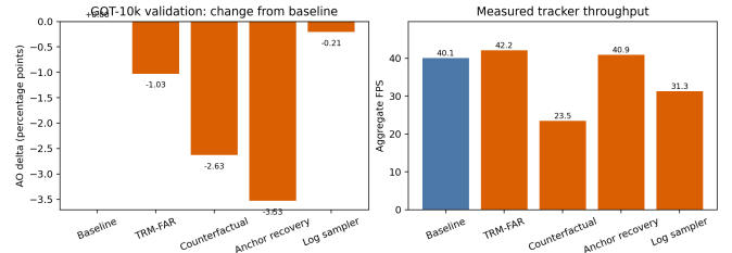
Fig. 2. Measured complete GOT-10k validation outcomes. Orange bars are rejected candidate mechanisms; the graphic reports observed B_{\text{dev}} data only and is not a held-out benchmark result.
