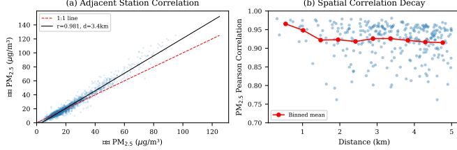
Fig. 4. (a) Scatter plot of \text{PM}_{2.5} readings for the highest-correlation adjacent station pair. (b) Spatial correlation decay: \text{PM}_{2.5} correlation vs. inter-station distance for 279 pairs within 5 km.
