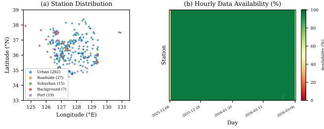
Fig. 1. (a) Spatial distribution of 350 AirKorea stations by type. (b) Hourly data availability for 50 representative stations over the study period.
