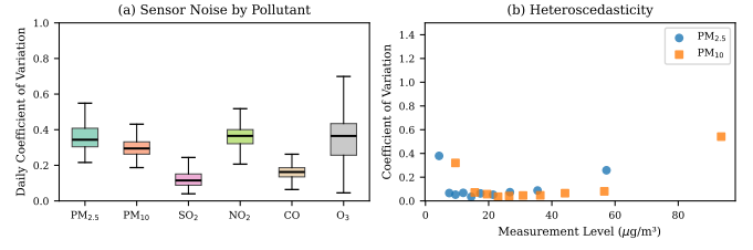
Fig. 2. (a) Distribution of daily CV across stations for each pollutant. (b) Heteroscedasticity: CV as a function of concentration level for PM 2.5 and PM 10 .
