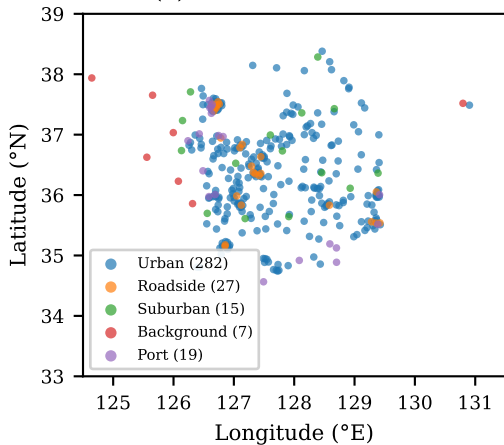
(a) Station Distribution
