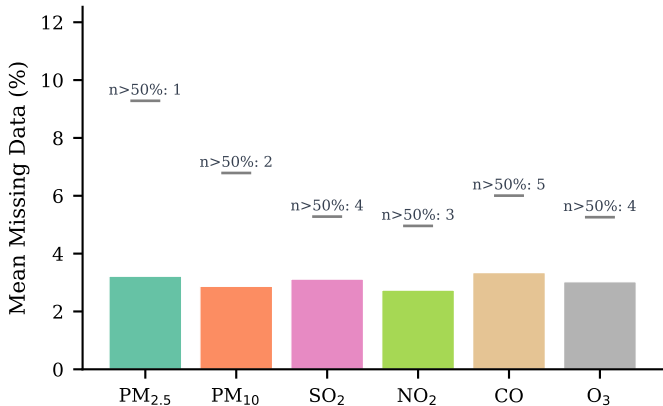
(b) Data Missingness by Pollutant (cap = 95th pct; labels = stations >50% missing)
