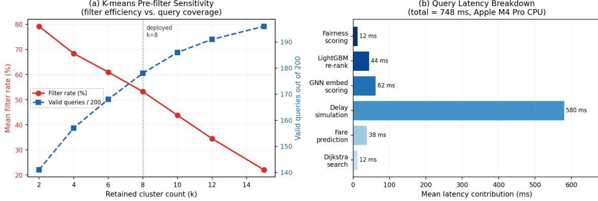
Figure 3: System analysis. Left: K-means pre-filter sensitivity — filter rate (%) and valid query count as a function of retained cluster count k_{\text{retain}} (out of 20 total clusters). The deployed value k_{\text{retain}} = 8 (53.2% filter, 178/200 valid queries) sits at the elbow of the coverage–efficiency curve. Right: query latency breakdown showing that Monte Carlo delay simulation (580 ms) dominates the 748 ms total; Dijkstra search contributes only 12 ms.
