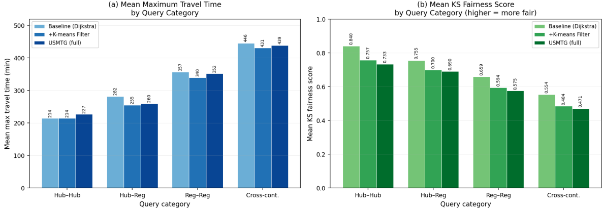
Figure 2: Ablation study results visualised as grouped bar charts. Left: mean maximum travel time per query category (lower is better). Right: mean KS fairness score per category (higher is more equitable). The baseline achieves lower max-time but USMTG provides richer information at a 3.9% time overhead.
