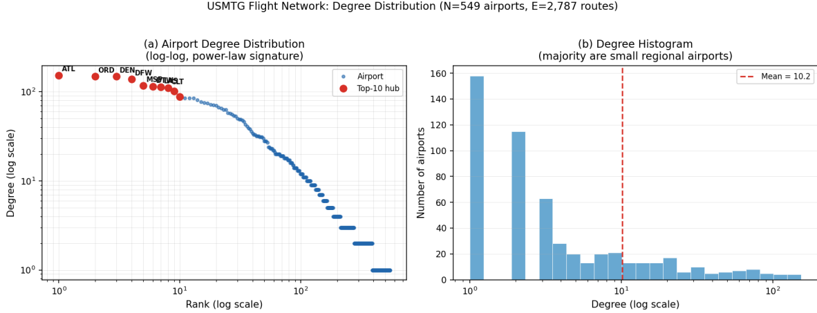
Figure 1: Degree distribution of the USMTG airport network. Left: log-log rank plot showing a power-law-like tail consistent with scale-free network models [7, 27]. Right: degree histogram confirming that the majority of airports are small regional nodes ( \delta < 20 ) while a handful of major hubs ( \delta > 100 ) anchor the network.
