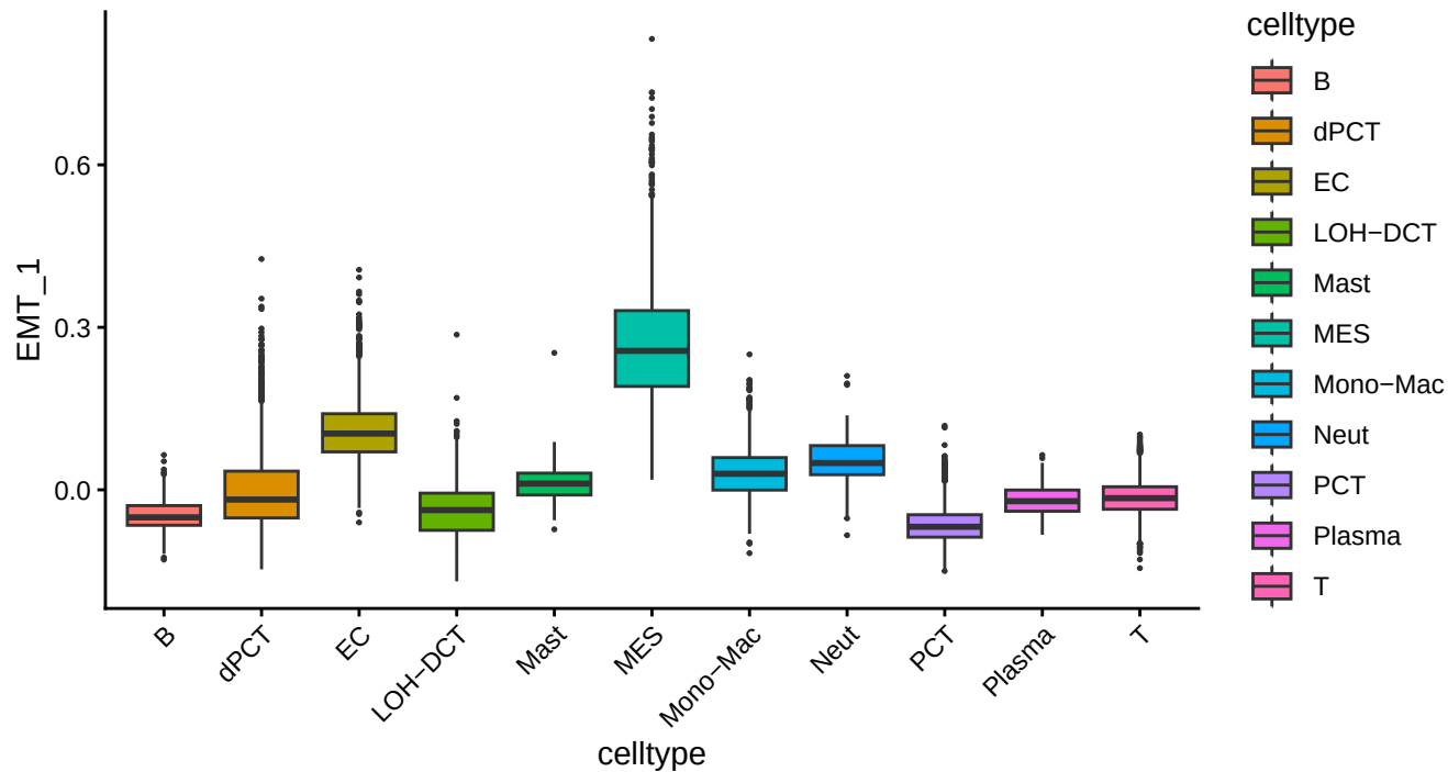
EMT module score by cell type
