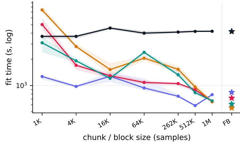
CPU · fit time vs chunk
