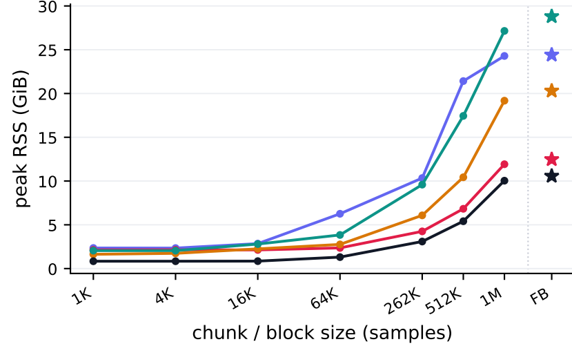
CPU · peak memory vs chunk
