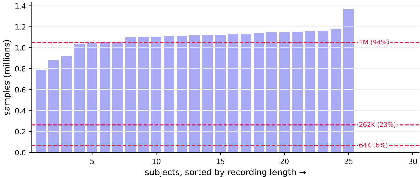
Per-subject recording length (ds004505, 25 subjects @250 Hz) vs the tested chunk sizes
