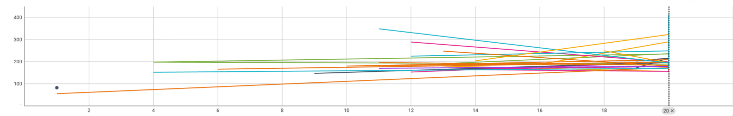
Stylization/Input
