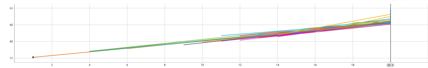
Stylization/GenerationTime
