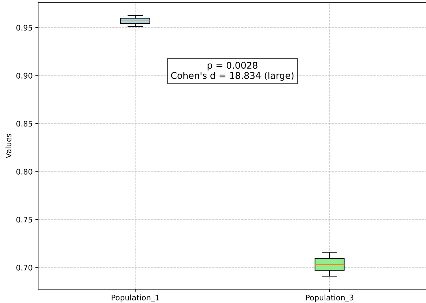
Comparison between Population_1 and Population_3
