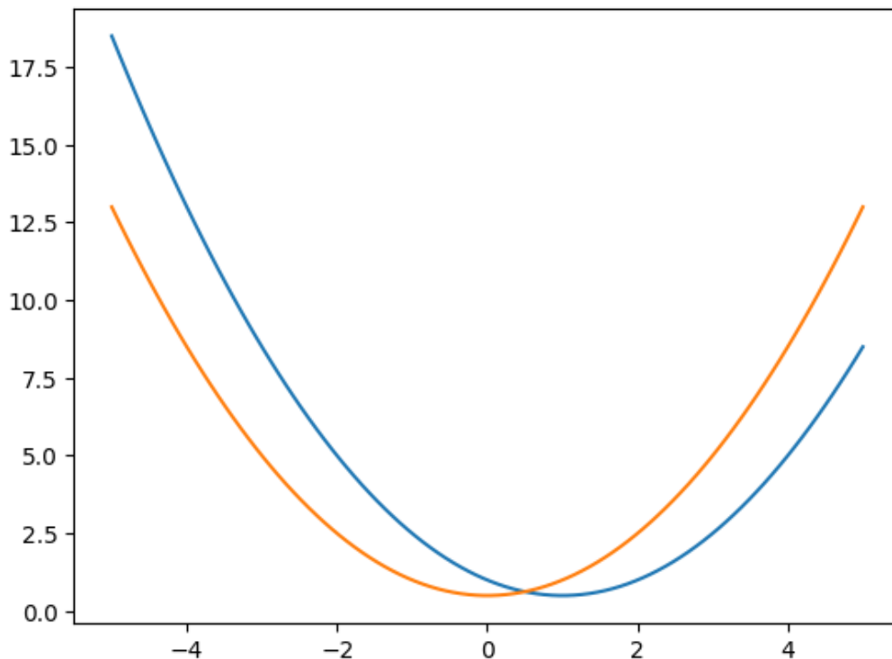
図 4.6 Notebook figure 03-06
