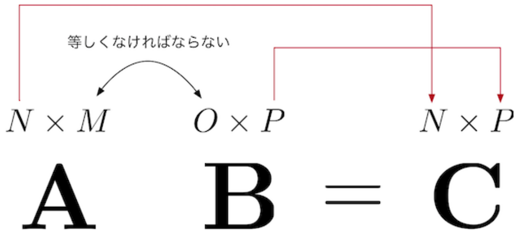
図 7.3 matrix product
