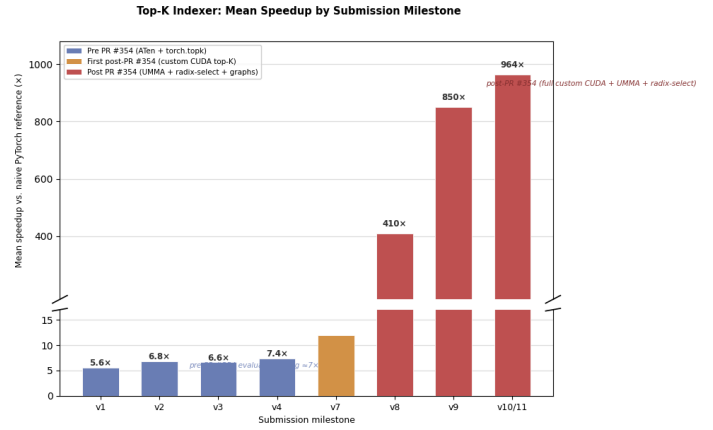
Figure 1. Indexer mean speedup vs. the naive PyTorch reference, by submission milestone. The flat plateau at v1–v4 reflects the pre-PR #354 evaluator cap (~7×); the cliff at v7–v8 follows the full UMMA + radix-select rewrite; the final ~13% from v9 to v11 comes from CUDA-graph overhead elimination on the small-workload bucket.
