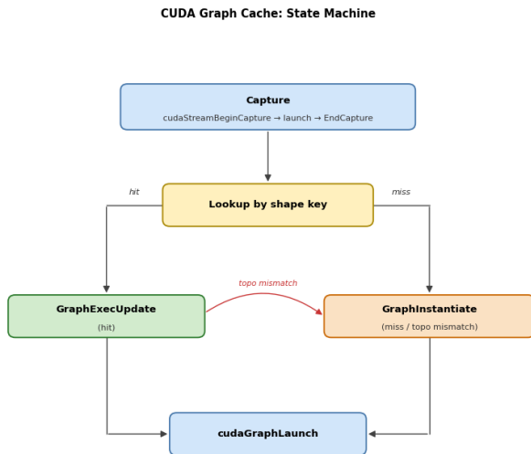
Figure 5. CUDA-graph cache state machine. On every call we capture the current launch sequence into a graph, look up the cached executable by shape key, and either redirect node pointers in-place via cudaGraphExecUpdate (hit) or instantiate a fresh executable (miss / topology mismatch); the executable is then replayed via cudaGraphLaunch .
