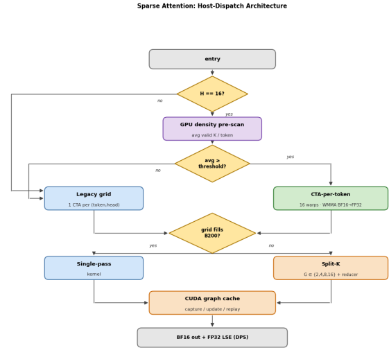
Figure 4. Sparse Attention dispatch architecture: an H == 16 predicate gates a GPU density pre-scan; high-density shapes use a CTA-per-token WMMA path, low-density shapes fall back to the legacy grid; an underfill check then routes between a single-pass kernel and a split-K kernel with reducer; all paths terminate in a CUDA-graph-cached launch sequence.
