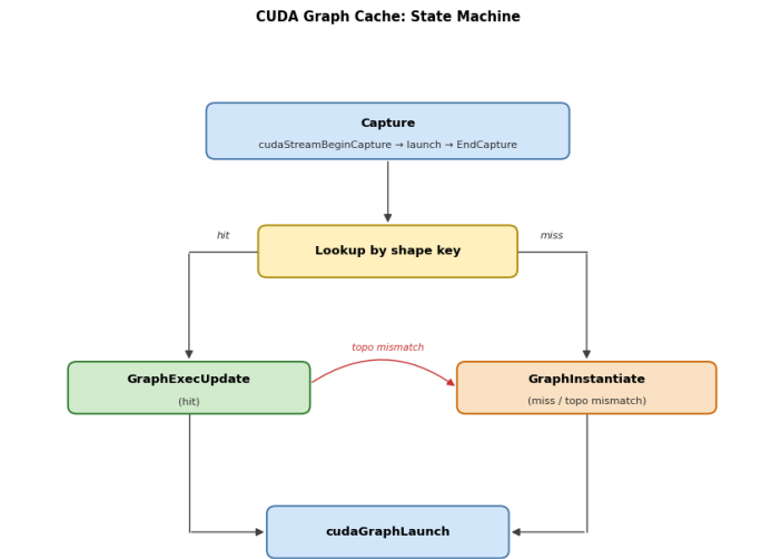
Figure 5. CUDA-graph cache state machine. On every call we capture the current launch sequence into a graph, look up the cached executable by shape key, and either redirect node pointers in-place via cudaGraphExecUpdate (hit) or instantiate a fresh executable (miss / topology mismatch); the executable is then replayed via cudaGraphLaunch .
