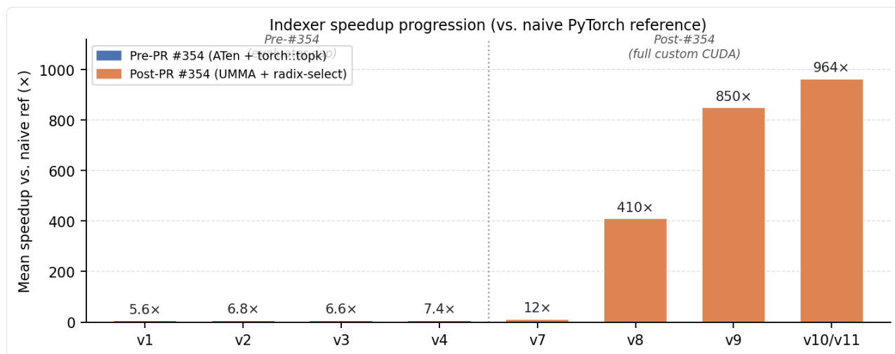
Figure 1. The flat plateau at v1–v4 corresponds to the period when the old evaluator capped progress; the sharp rise at v7–v8 follows PR #354 and the UMMA + radix-select rewrite; the final 13% from v9 to v11 comes from CUDA-graph overhead elimination.
