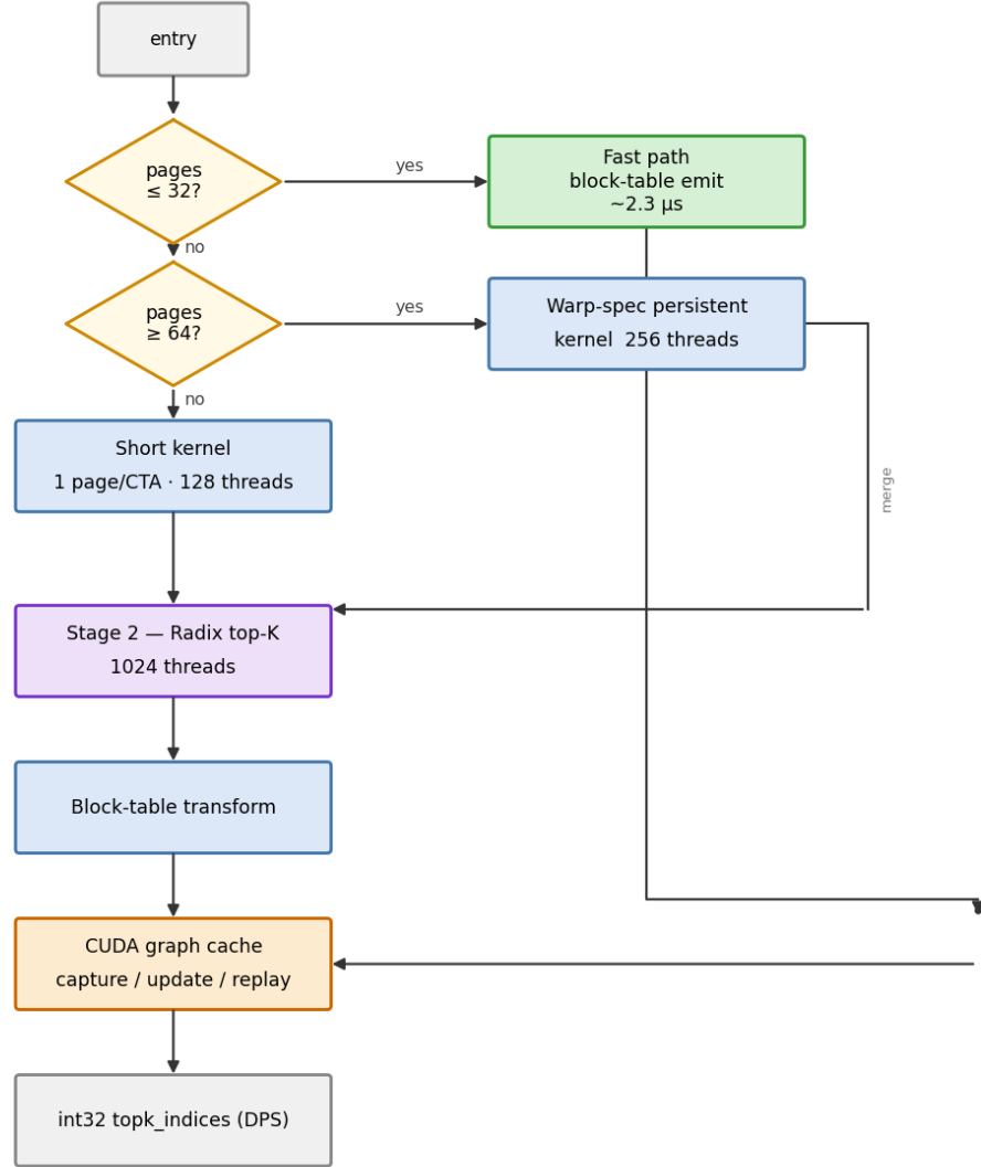
Figure 2. Top-K Indexer dispatch architecture
