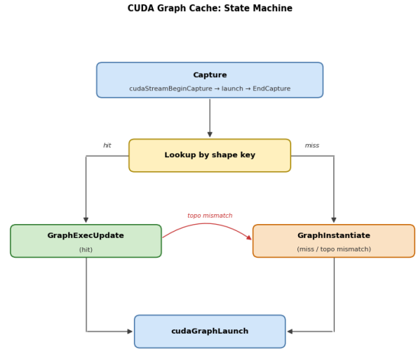
Figure 6. CUDA-graph cache state machine. On every call we capture the current launch sequence into a graph, look up the cached executable by shape key, and either redirect node pointers in-place via cudaGraphExecUpdate (hit) or instantiate a fresh executable (miss / topology mismatch); the executable is then replayed via cudaGraphLaunch .
