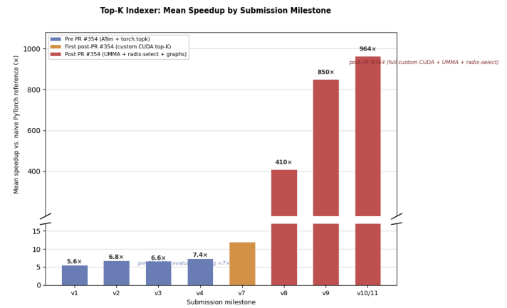
Figure 2. Indexer mean speedup vs. the naive PyTorch reference, by submission milestone. The flat plateau at v1–v4 reflects the pre-PR #354 evaluator cap ( \approx 7\times ); the cliff at v7–v8 follows the full UMMA + radix-select rewrite; the final \approx 13\% from v9 to v11 comes from CUDA-graph overhead elimination on the small-workload bucket.
