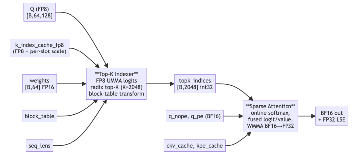
Figure 1. DSA decoding pipeline dataflow. Inputs to the Top-K Indexer ( FP8 query, paged KV cache with per-slot scales, attention weights, block table, sequence lengths) flow through UMMA-based logit scoring and radix top-K selection to produce topk_indices of shape B \times 2048 . The Sparse Attention kernel consumes those indices together with BF16 query tensors and compressed KV caches to produce BF16 output and FP32 LSE in destination-passing style.
