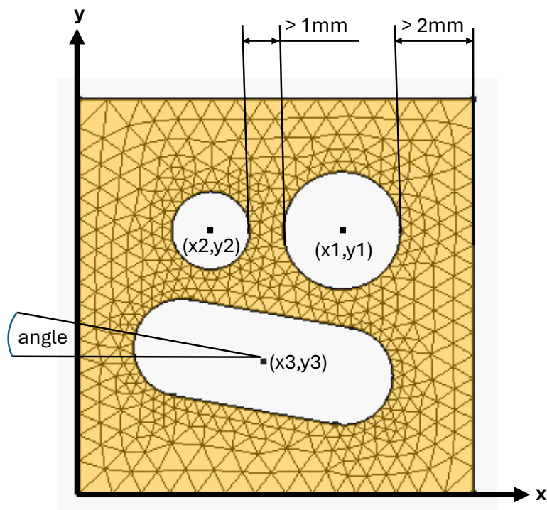
Figure 1: Geometry to optimize with indicated design variables
