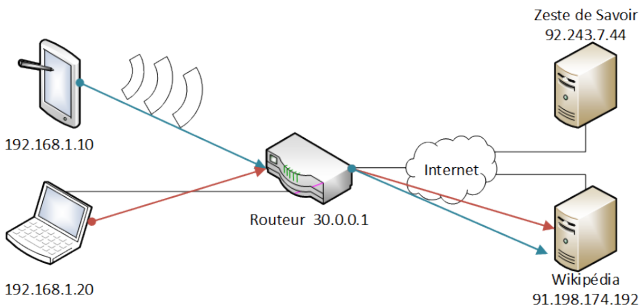
FIGURE VI.3.4. – Translation de ports
