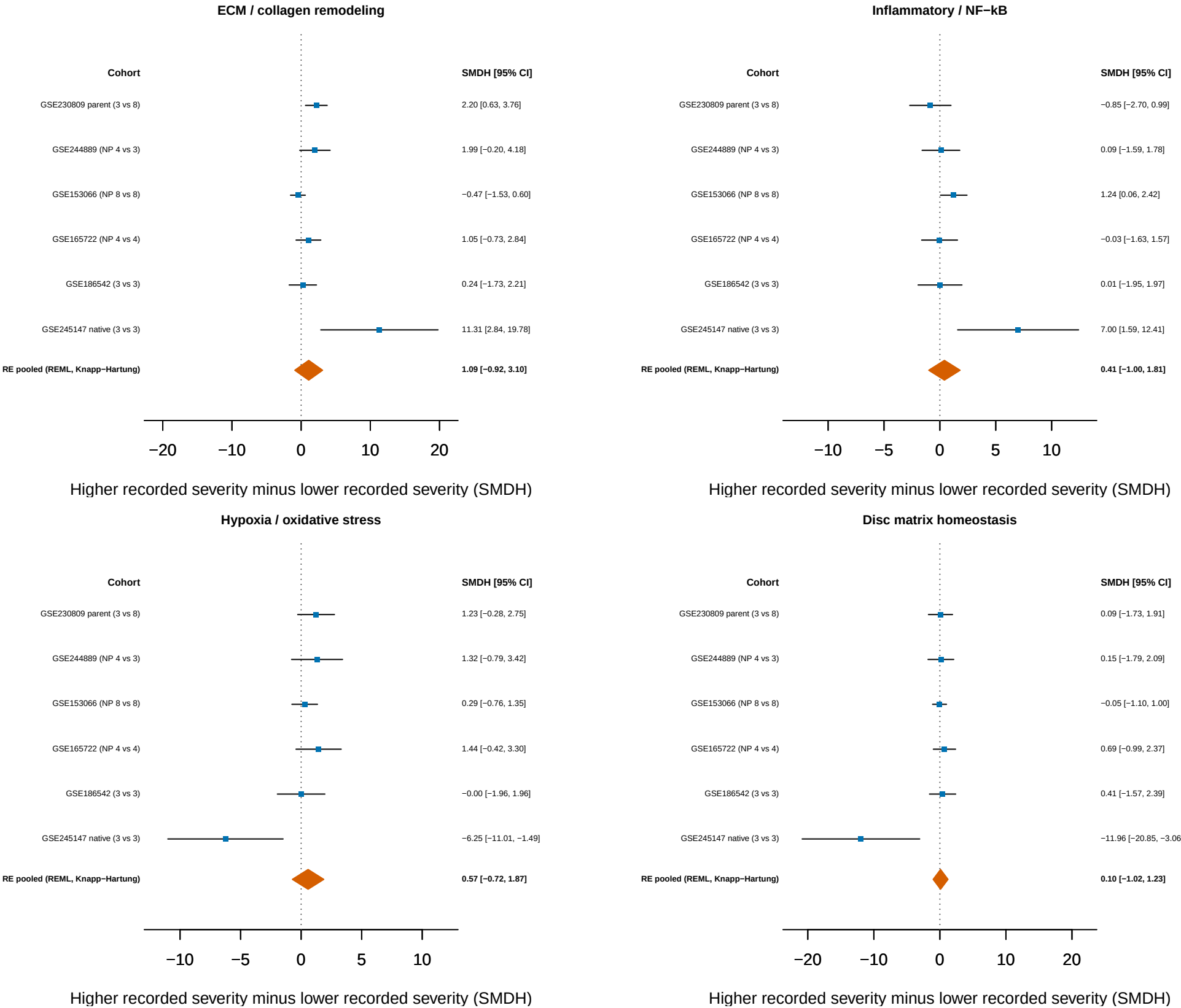
Supplementary Figure S5. Source–family replacement sensitivity for the post hoc NP random–effects synthesis.
