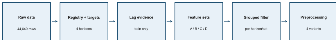
Figure 4.1. Leakage-controlled feature-preparation pipeline generated by Notebook 02.
