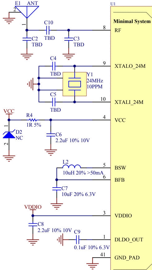
FR8008AP_QFN40_0505
