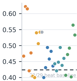
OWL lower is better
