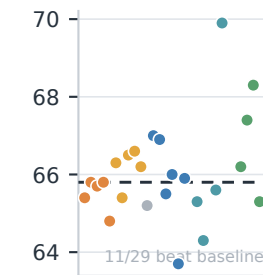
DiGress lower is better
