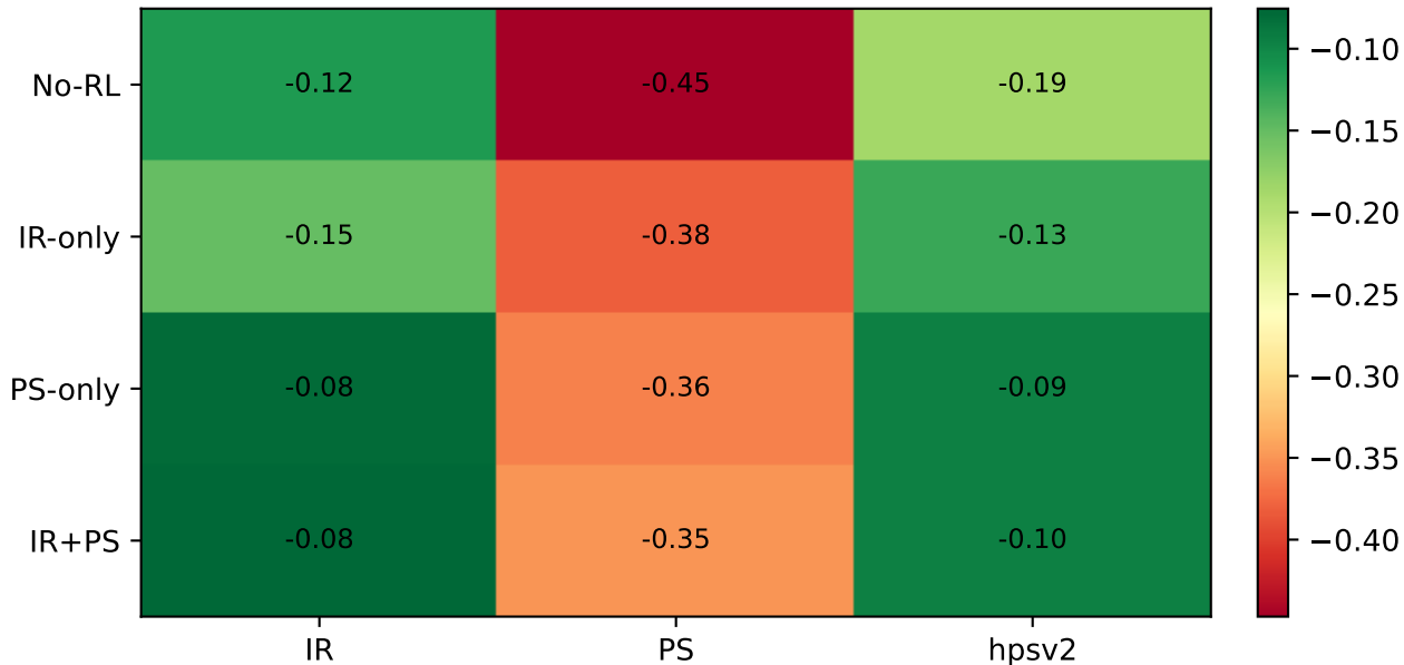
Final cross-reward matrix (calibrated z)
