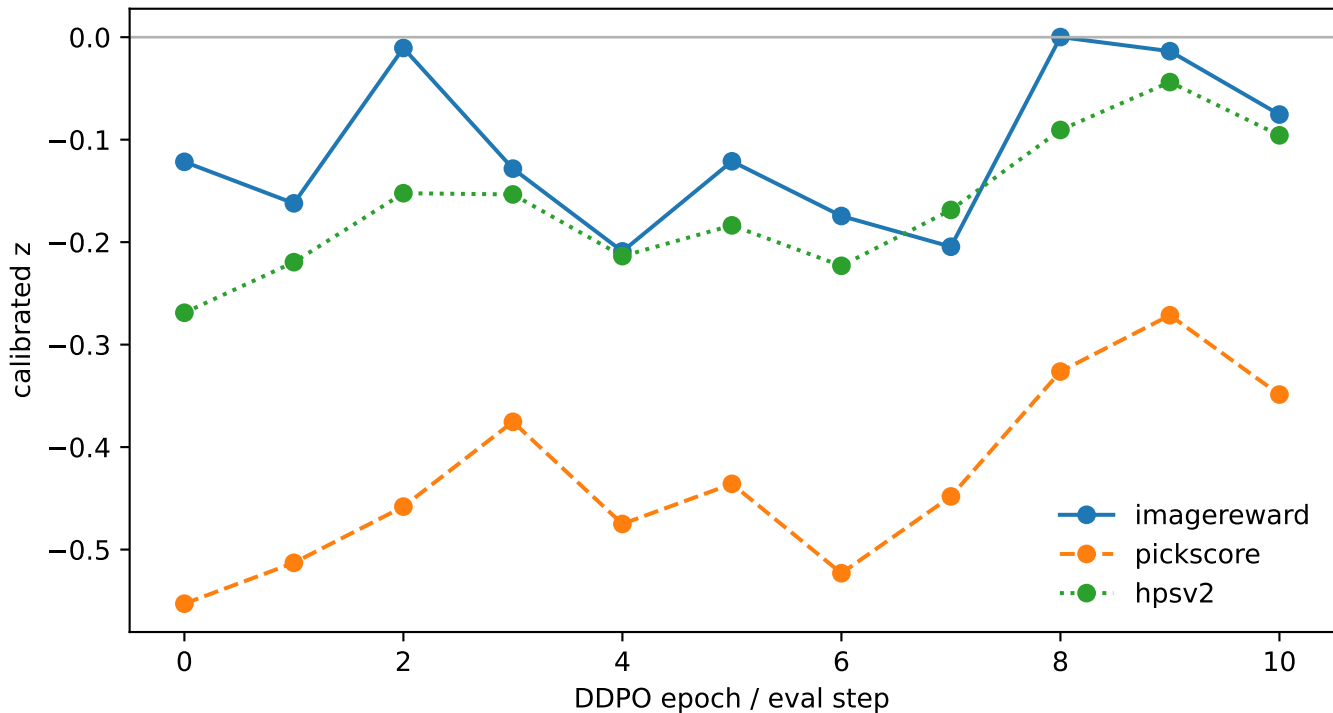
IR+PS cross-reward trajectory
