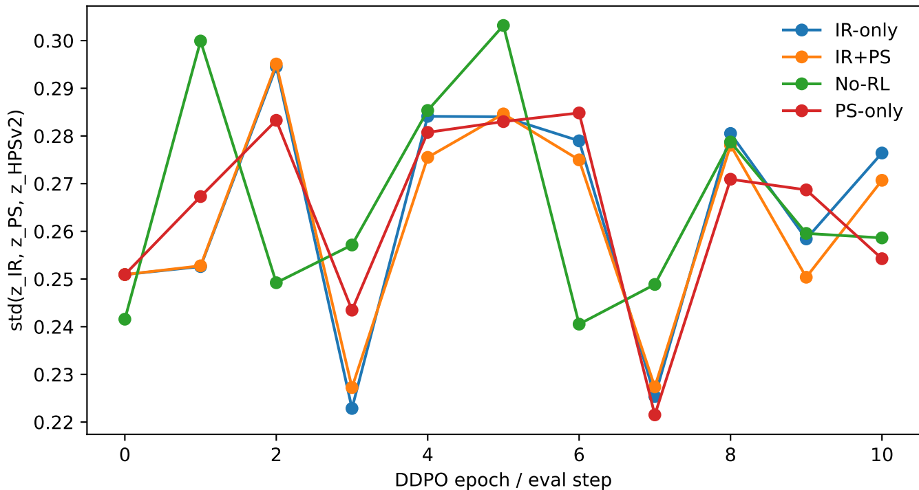
Reward disagreement
