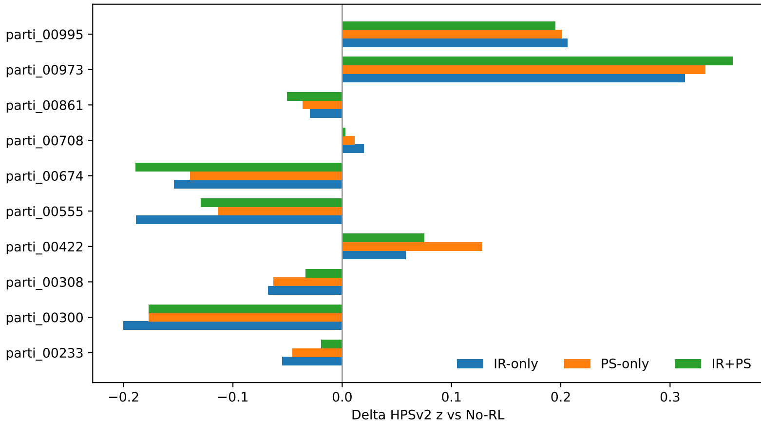
Per-prompt held-out reward delta (all rollouts)
