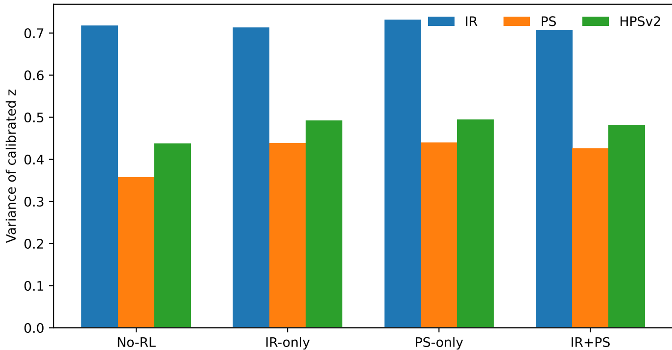
All-rollout reward variances
