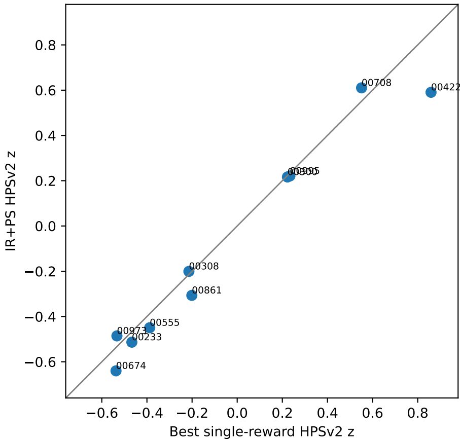
IR+PS vs best single reward per prompt
