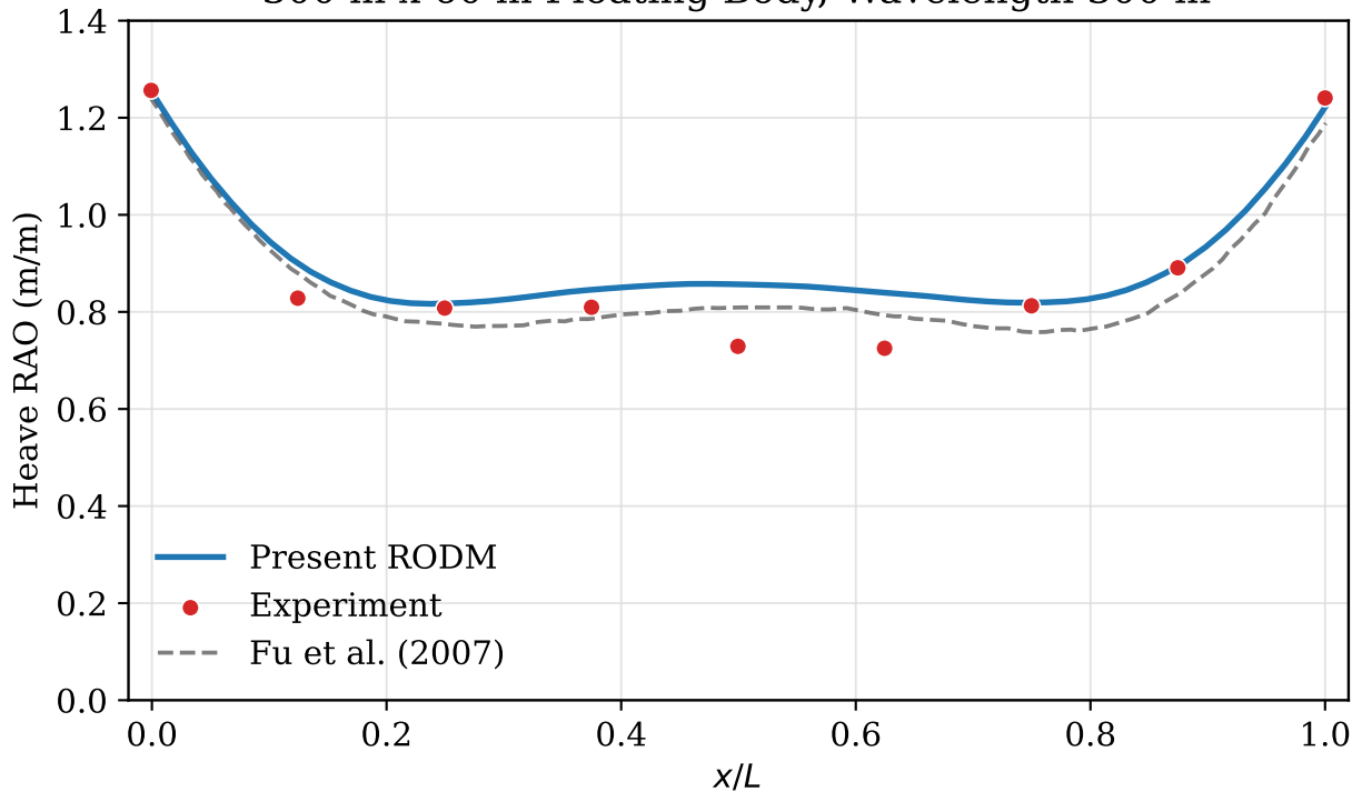
300 m x 60 m Floating Body, Wavelength 300 m
