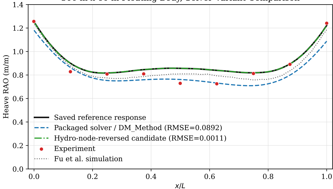
300 m x 60 m Floating Body, Solver Variant Comparison
