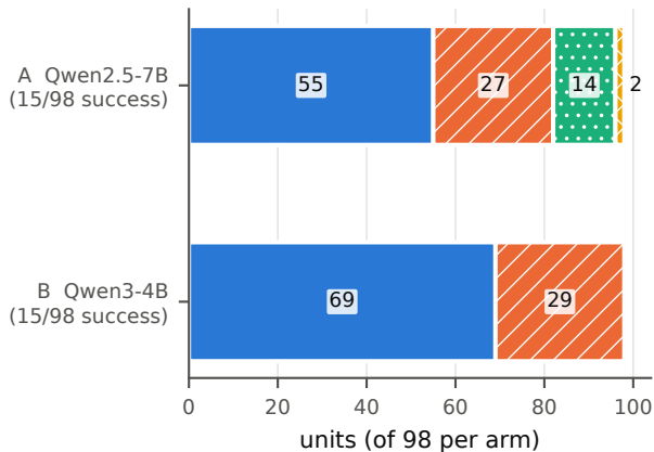
termination reason (timeout: 0 in both arms)
