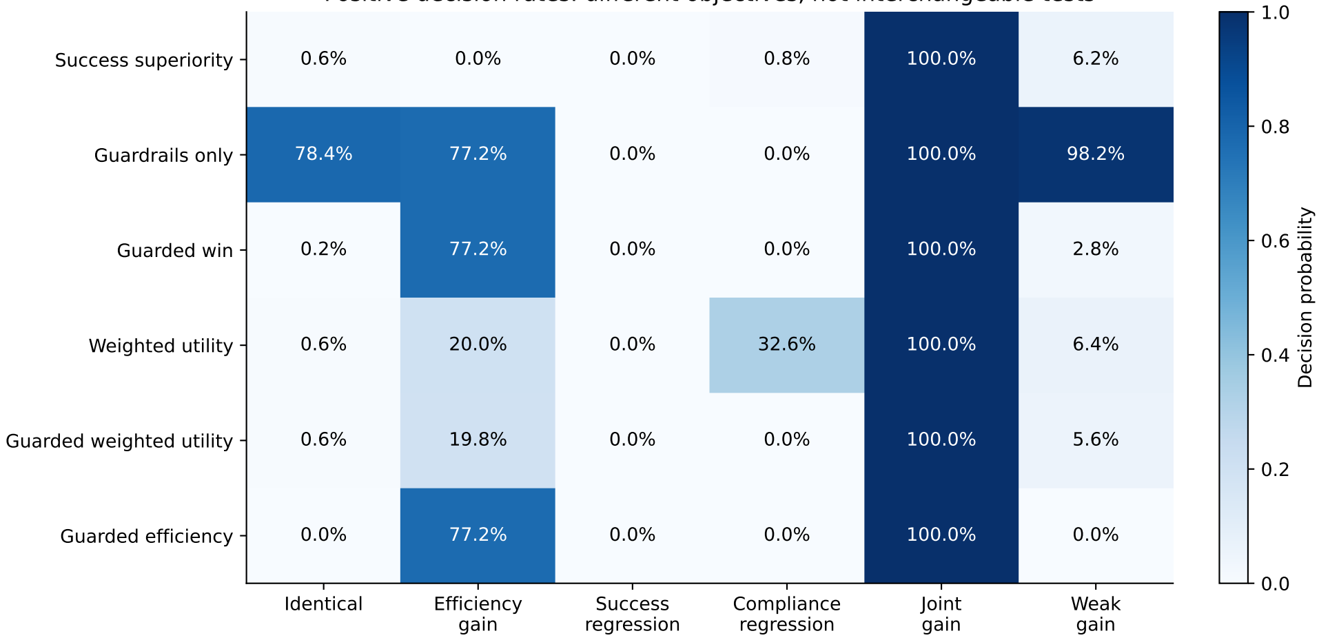
Positive decision rates: different objectives, not interchangeable tests
