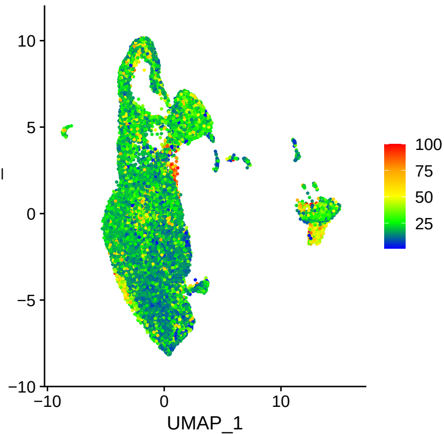
percent.mt
