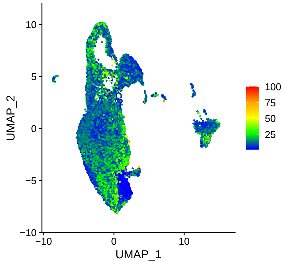
nCount_RNA
