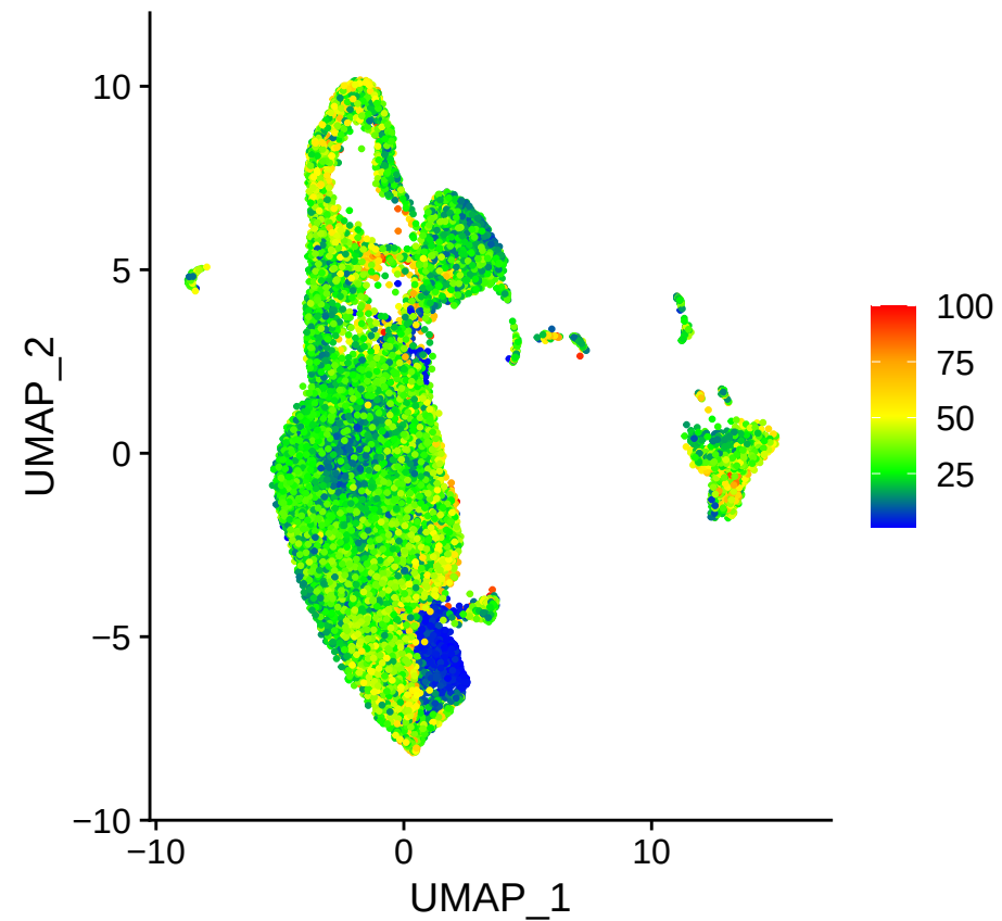
nFeature_RNA
