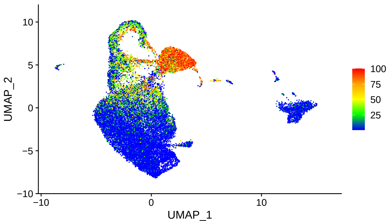
COL17A1
