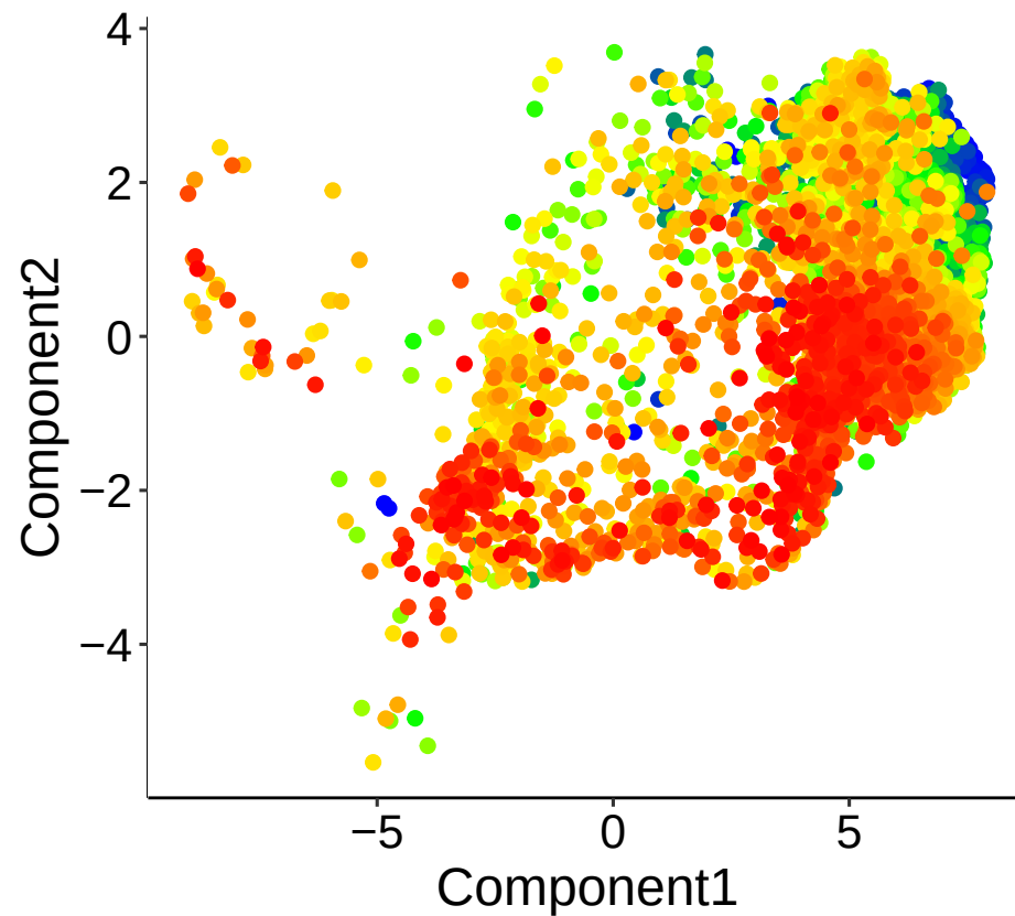
CytoTRACE
