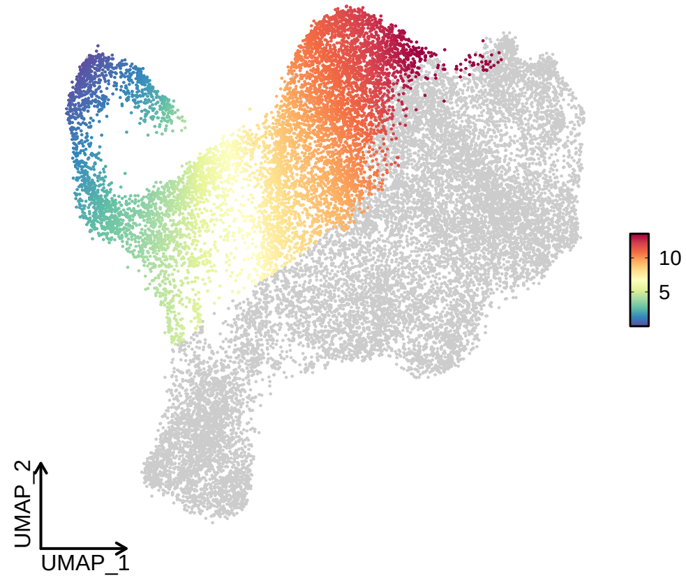
Lineage3
