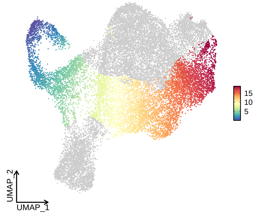
Lineage4
