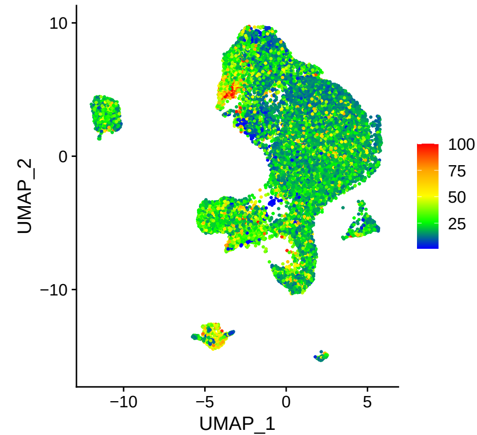
percent.mt
