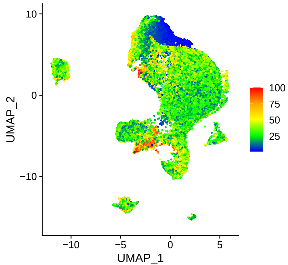
nFeature_RNA
