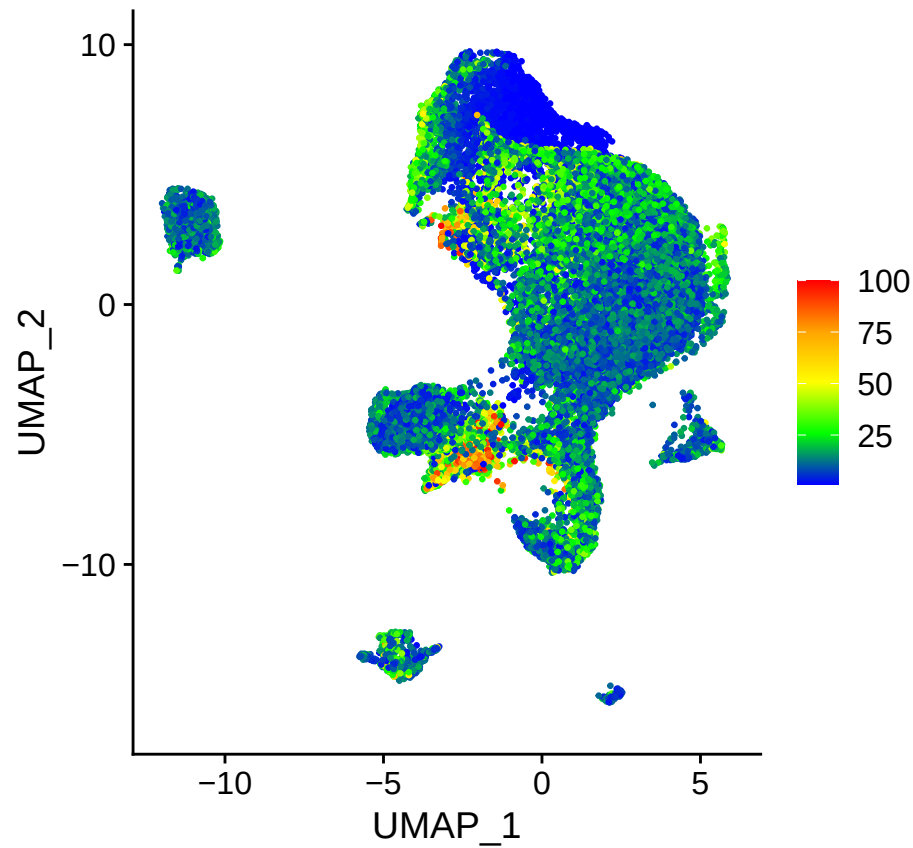
nCount_RNA
