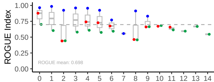
ROGUE index for res_0.5
