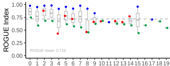
ROGUE index for res_0.9
