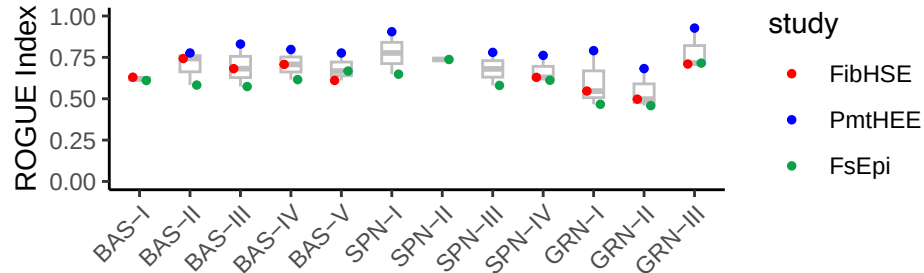
ROGUE index for cell_type
