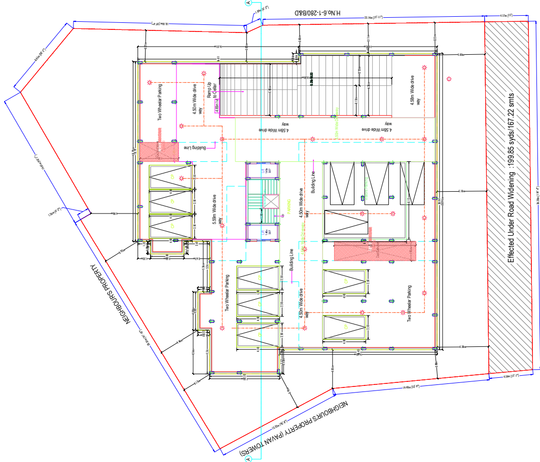
SUB-CELLAR FLOOR PLAN (SCALE 1:100)
