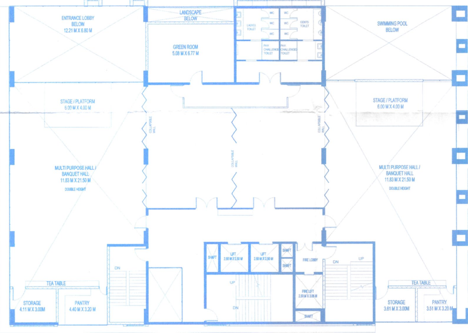
FIRST FLOORPLAN
