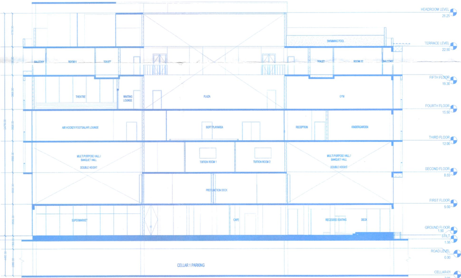
SECTION-CC'
