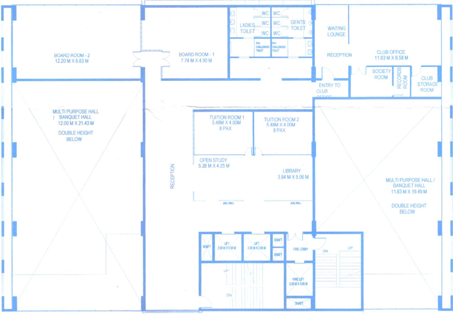
SECOND FLOORPLAN
