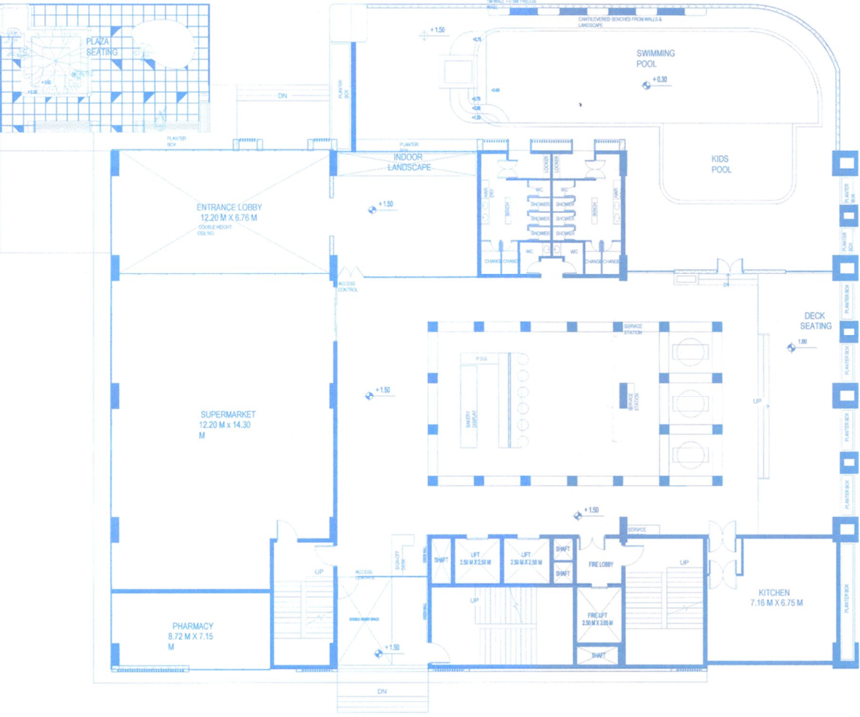
GROUND FLOORPLAN
