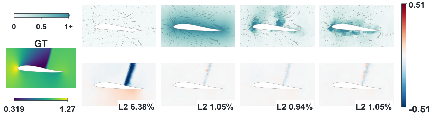
Airfoil2D
