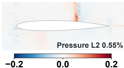
Prediction - CFD
