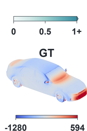
DrivAerML
