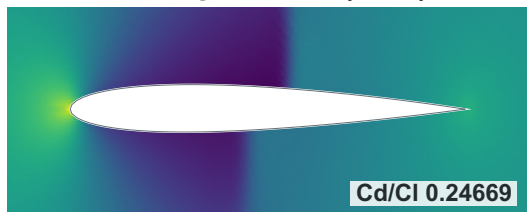
Initial pressure (CFD)
