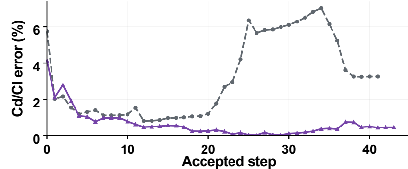
Prediction vs. CFD
