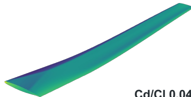
Final pressure (CFD)
