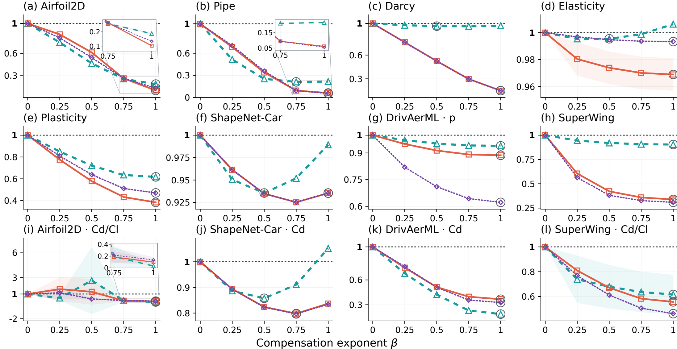
Error-budget area ratio R_m(\beta)
