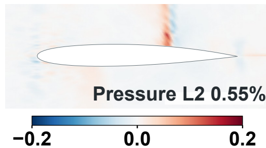
Prediction - CFD
