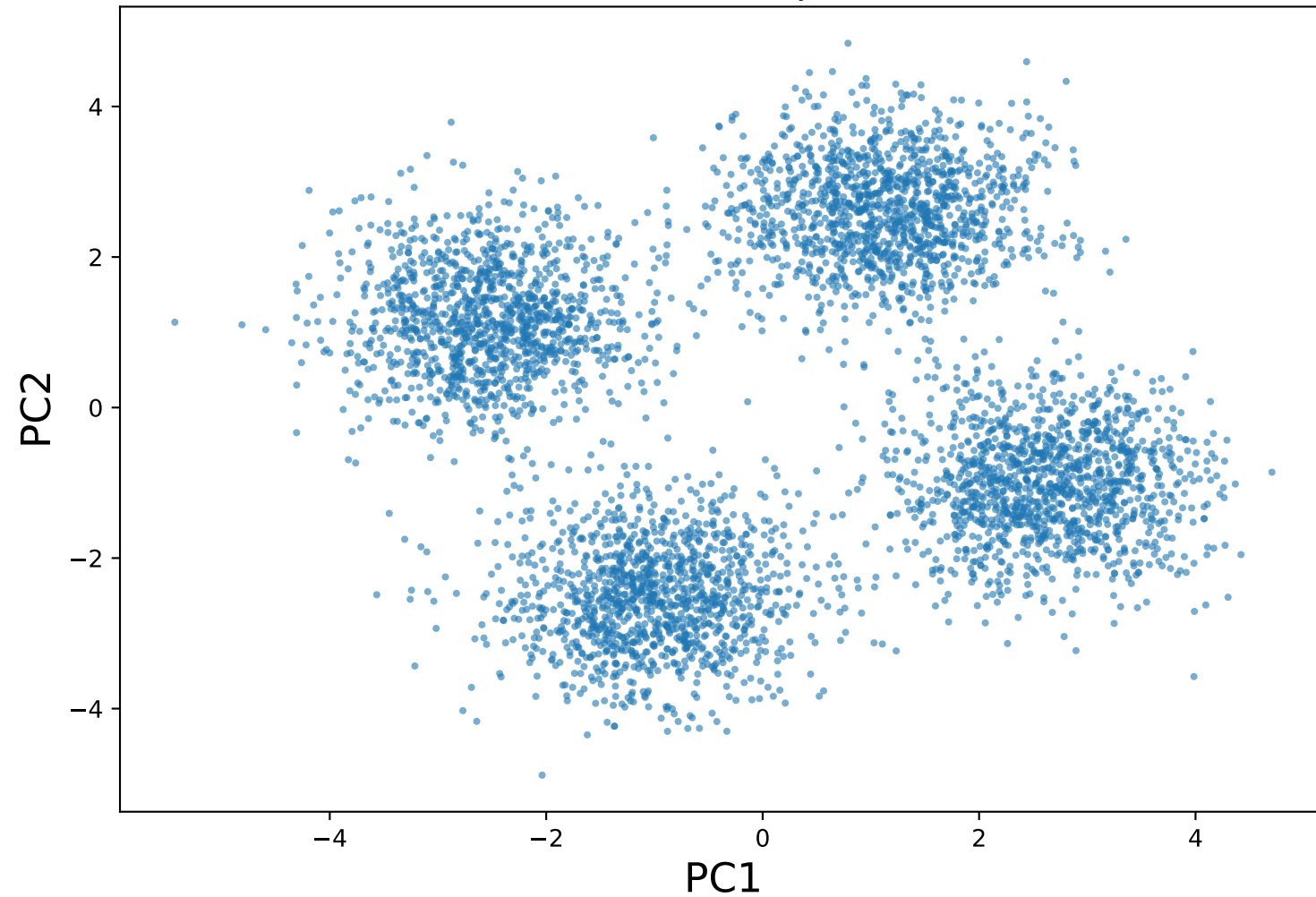
Generated Sample(PCA)
