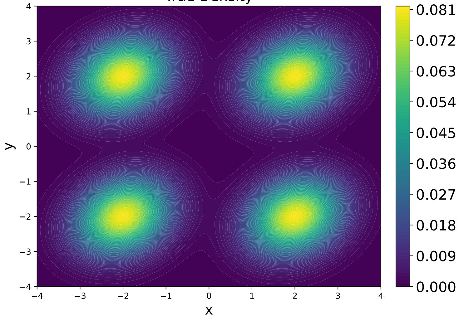
True Density
