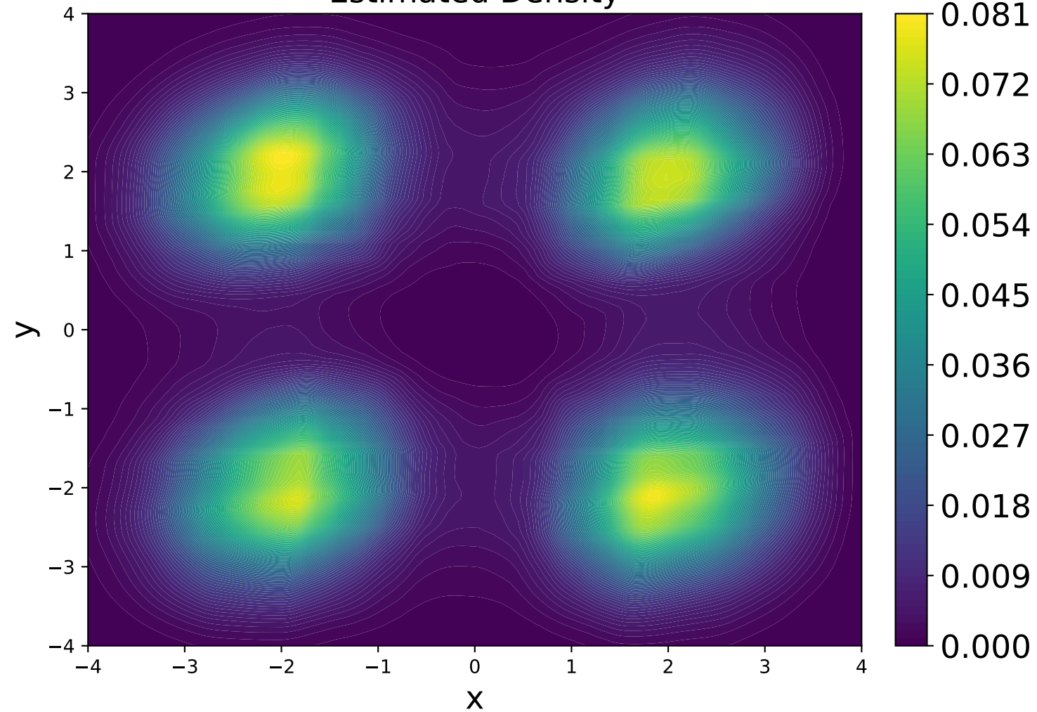
Estimated Density
