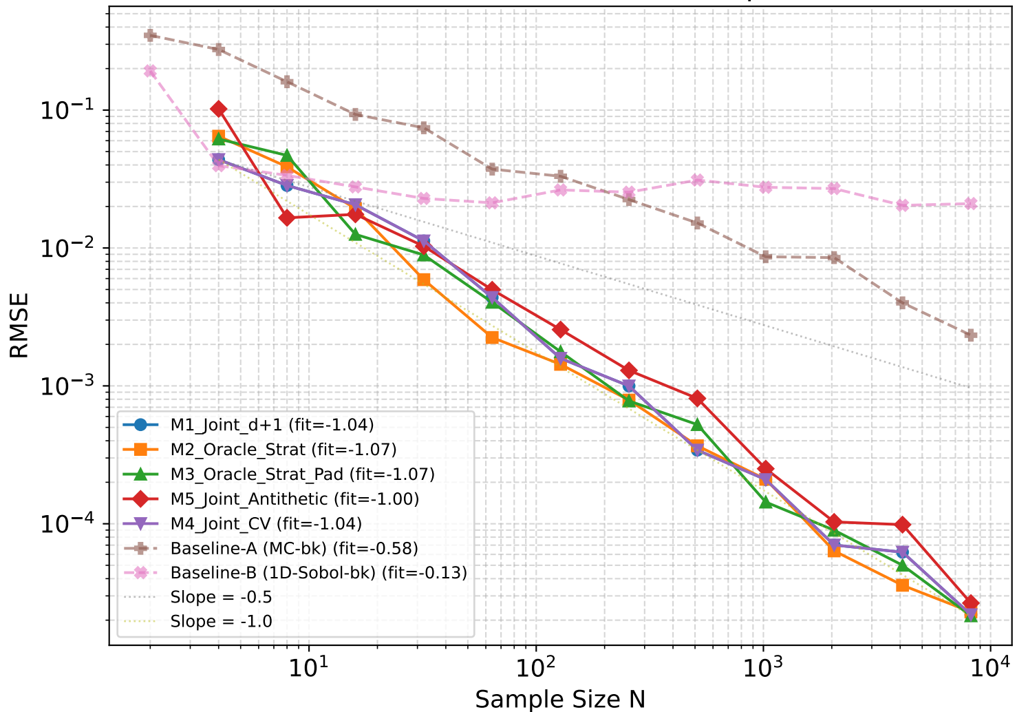
2D GMM advanced RQMC: Complex f
