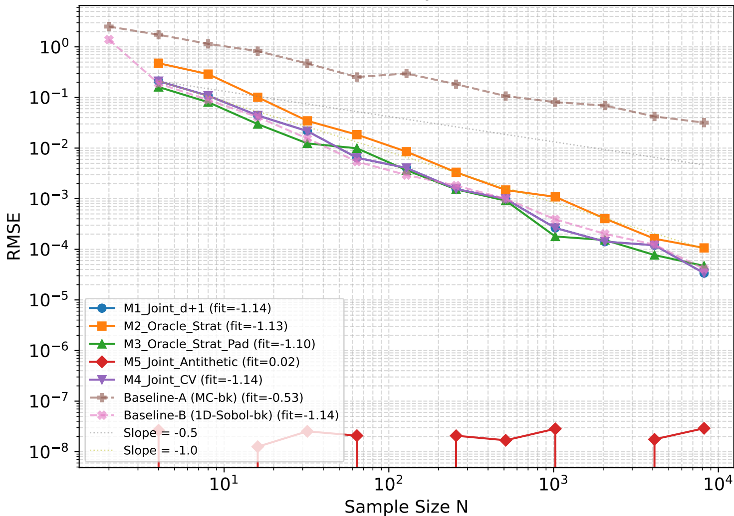
2D GMM advanced RQMC: First moment
