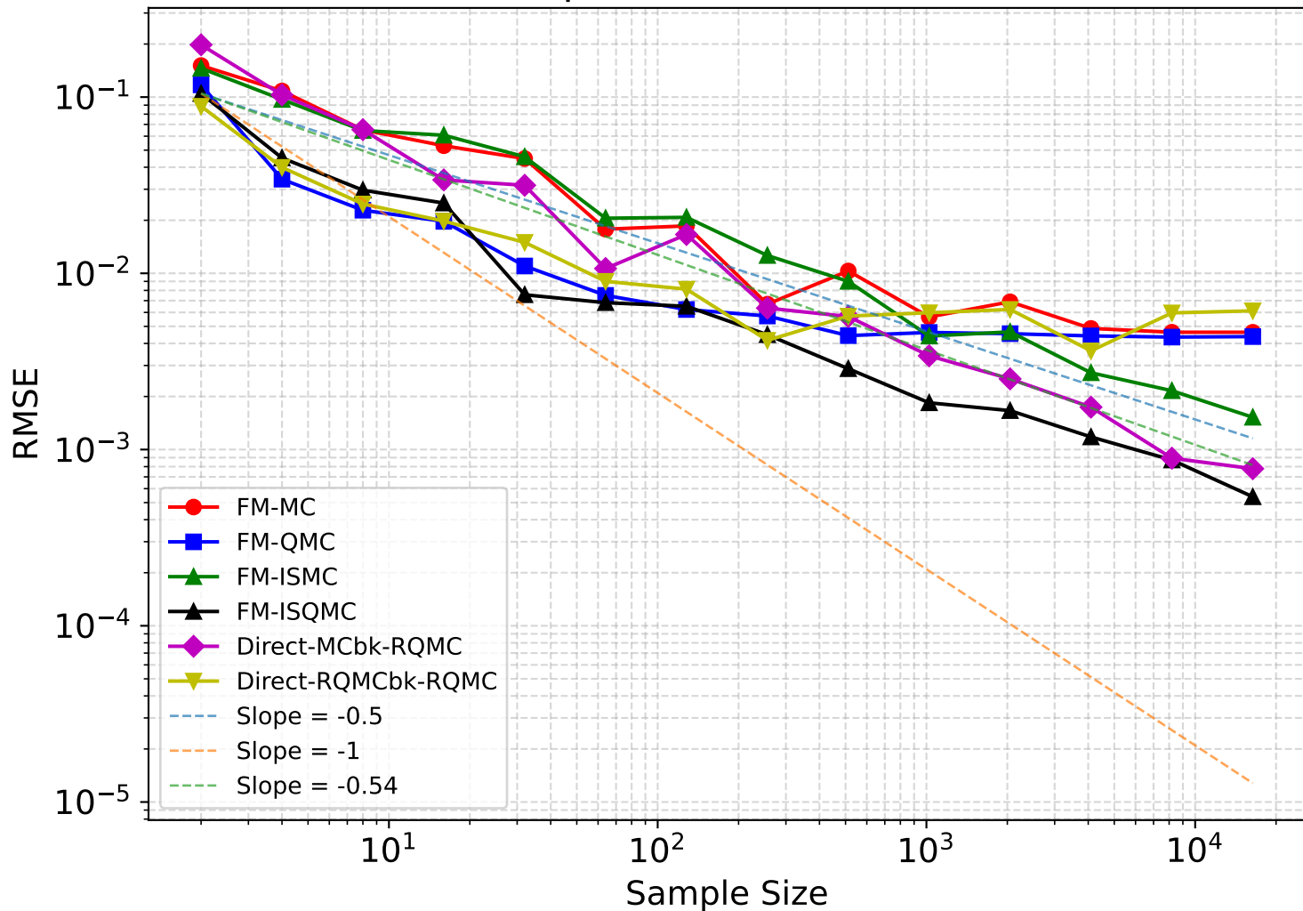
30D GMM, Complex f: 4 FM + 2 direct baselines
